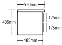
WINDOW SEAT 2 DRAWERS
