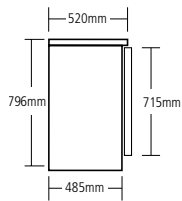
STANDARD CABINET
