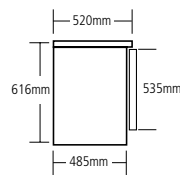
BEDSIDE CABINET
