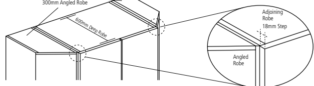
300MM ANGLED ROBE WITH 400MM DOOR. [STATE LH OR RH]
